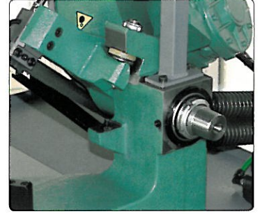
Cam for bow square adjustment
