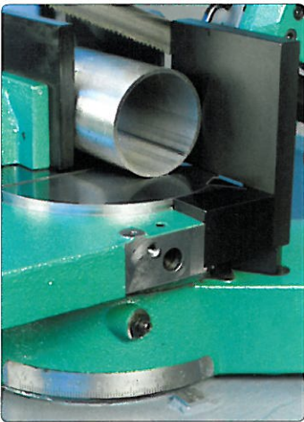
(*) Retractable vice shoulders to reach maximum cutting capacity (340 x 180 mm). Easy reading of engraved graduated scale
