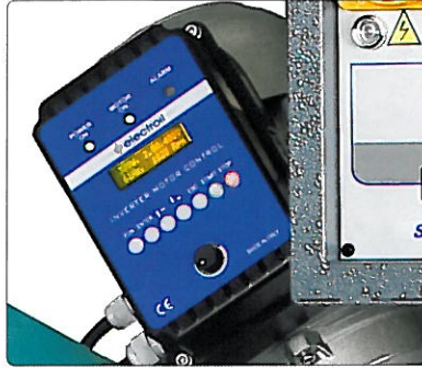
Electronic blade speed variator
